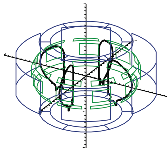
Fig. 2. ITER 3x9 RMP (green) and 3x6 EFC (blue) coil sets. ITER limiter is shown in black.
