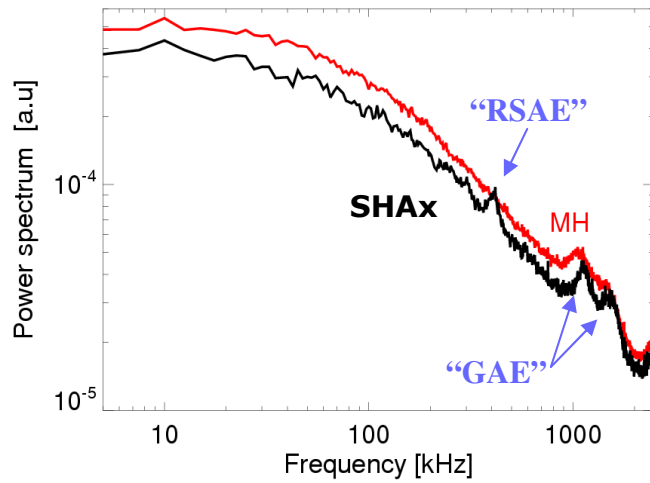
Fig. 5: Power spectra of \dot{B}_p for the different topologies.
