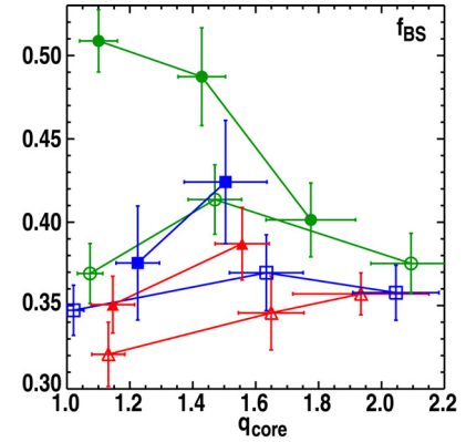
Fig. 1. Calculated bootstrap current fraction. \beta_N=2.8 (open), maximum beam power (closed), q_{95} : 4.5 (triangles), 5.6 (squares), 6.8 (circles). q_{\text{core}} is the average value of q in the region 0.0 < \text{normalized radius } \rho < 0.3 .
