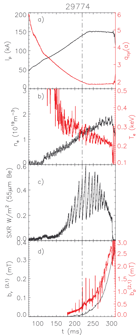
Fig.1) a) Plasma current and q_{cyl}(a) ; b) electron density and temperature; c) SXR signals; d) radial and poloidal (2,1) harmonics
