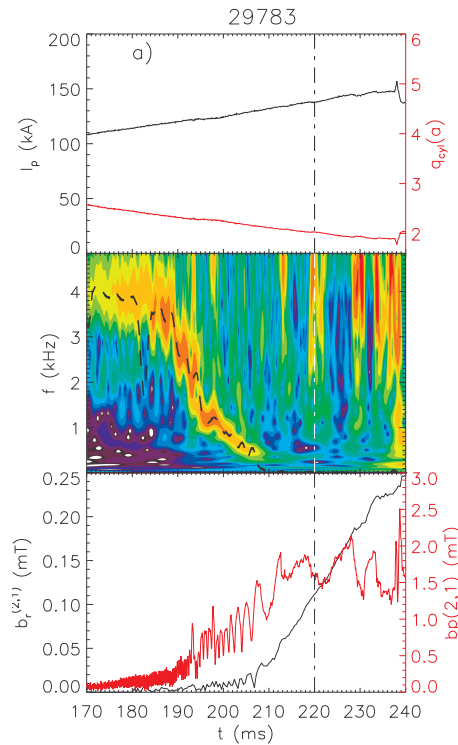
Fig. 2a) Plasma current and q_{cyl}(a) ; b) wavelet spectrum of internal b_p ; c) radial and poloidal (2,1) harmonics
