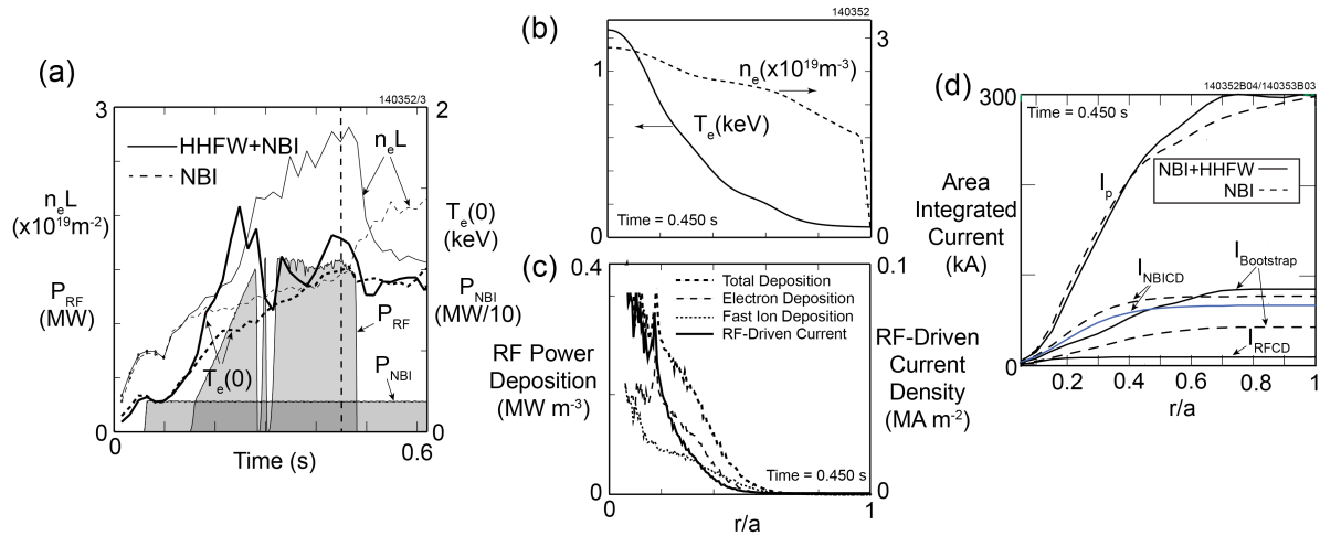
Fig. 3. (a) Time evolution of T_e(0) and n_e L for two similar I_p = 300 kA NBI H-modes, one with P_{\text{RF}} = 1.4 MW and P_{\text{NBI}} = 2 MW (solid lines, shot 140352), and the other with only P_{\text{NBI}} = 2 MW (dashed lines, shot 140353). (b) T_e(r/a) and n_e(r/a) , and (c) RF deposition and RF-driven current calculated by GENRAY-ADJ for P_{\text{RF}} = 1 MW, at 0.450 s during shot 140352. (d) Area integrated I_p , I_{\text{NBICD}} , I_{\text{Bootstrap}} , and I_{\text{RFCD}} versus r/a calculated at 0.450 s by TRANSP-TORIC, assuming \eta_{\text{eff}} = 100\% .
