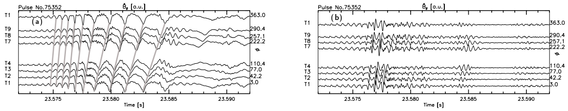
Figure 2: (a) Toroidal array of \dot{B}_\theta(t) coils. (b) Same signals high pass filtered with a cut-off frequency of 2kHz, in order to decrease the m/n = 2/1 component.
