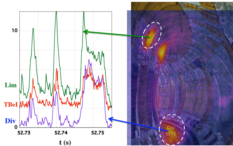
Figure 2: Beryllium emission image and time evolution
