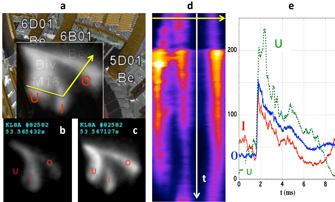
Figure 2: ELM dynamics study (see text for figure explanation).
