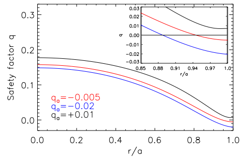
Figure 1: Radial profile of the safety factor q for a shallow (red line), a deep (blue line) and a positive (black) q_a discharge.
