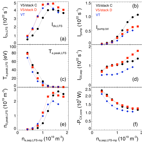
Fig.3 (a) I_{div,LFS} , (b) total pumped deuterium, I_{pump,tot} , (c) T_{e,peak,LFS-plate} , (d) total atomic deuterium current total ion current across separatrix, (e) peak neutral deuterium density in the LFS divertor leg, and (f) charge exchange loss power in the core as function of n_{e,sep,LFS-mp} .
