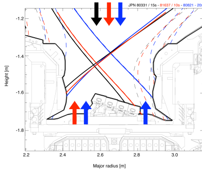
Fig.1 Separatrix and 2 cm flux surface (LFS midplane equivalent) for the V5/C (black), V5/D (red) and VT (blue) configurations.
