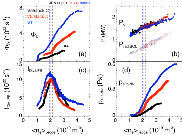
Fig.2 (a) Deuterium gas fuelling, (b) ohmic (solid symbols) and radiated power in the SOL (open), (c) total ion current to the LFS divertor plate, and (d) neutral pressure in the LFS subdivertor as function of \langle n_e \rangle_{l,edge} . The vertical lines indicate \langle n_e \rangle_{l,edge} at which I_{div,LFS} saturated.
