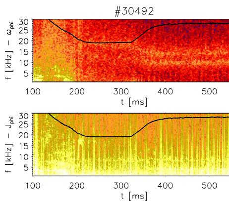
Fig. 5 J and \omega spectrograms, the time trace of q(a) is also shown (black line), measured at r/a=0.94(?) .
