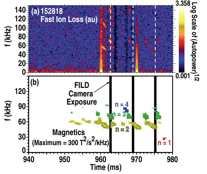
Figure 3: Spectrograms of (a) fast ion loss and (b) magnetic fluctuations for shot 152818. Vertical lines indicate the acquisitions of camera data from the FILD.
