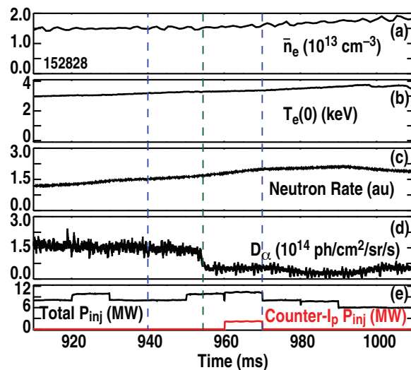
Figure 1: Time series data from shot 152828 including (a) line-averaged density, (b) central electron temperature, (c) neutron rate, (d) D_\alpha emission, and (e) injected neutral beam power.
