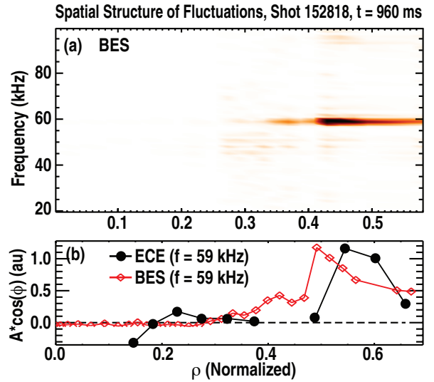
Figure 4: (a) Amplitude spectra (au) as a function of position for BES channels in shot 152818 at 960 ms. (b) Spatial profiles of fluctuation amplitude from the BES system ( \diamond -symbols) and ECE chords ( \bullet -symbols).
