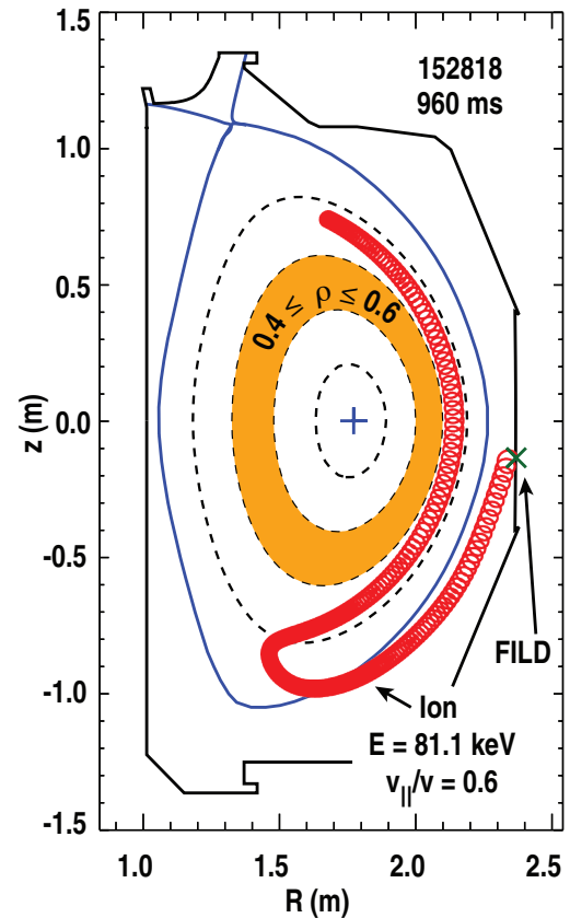
Figure 5: Magnetic equilibrium from shot 152818 at 960 ms. A back traced ion orbit using the FILD-measured E = 81.1 keV and v_{||}/v = 0.6 properties is shown.
