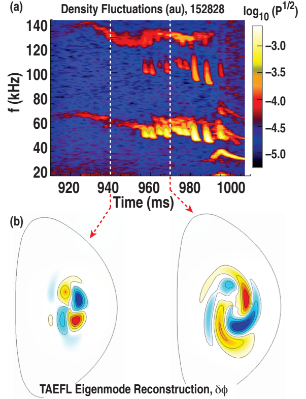
Figure 2: (a) Density fluctuations indicating the presence of strongly frequency chirping modes for t > 955 ms. (b) TAEFL calculations of the eigenmode structure at t = 940 ms and t = 970 ms. The last closed flux surface is shown for perspective (the minor radius is a = 60 cm).
