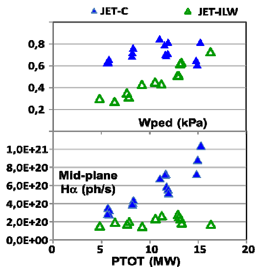
Fig 4: Comparison of i) pedestal energy and mid-plane recycling flux, for the power scan in the JET-C (blue triangles) and JET-ILW (green open triangle) for high triangularity.
