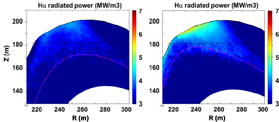
Fig 3: SOLEDGE2D EIRENE calculation for 2 hybrid discharges with different top clearance. The black rectangle represents the area of integration used in the measurement with the visible camera.
