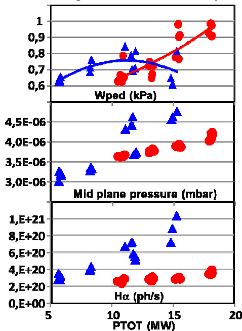
Fig 2: from top to bottom: i) energy content in the pedestal, ii) neutral, pressure in the main chamber, iii) H\alpha light from visible spectroscopy for high pulses (triangles) and low (dots) triangularity pulses of the power scan in JET-C.
