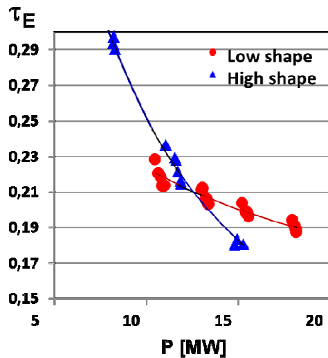
Fig 1: Confinement decay with power for the low shape (red dots) and high shape (blue triangles) triangles.
