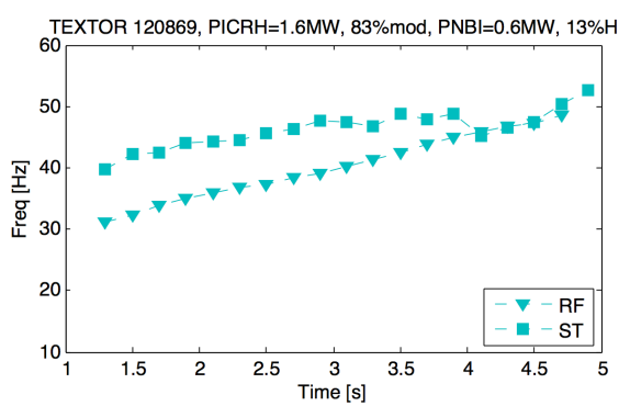
Fig. 3a: Fourier analysis of the locking of the sawteeth frequency with the ICRH modulation frequency
