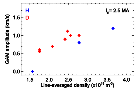
Figure 5: Dependence of the GAM amplitude on the plasma density for hydrogen and deuterium plasmas.
