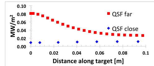
Fig. 4: Comparison of the power density calculated by TECXY at the outer target for the two QSF equilibria, n_{e,LCMS} = 3 \times 10^{18} m^{-3}
