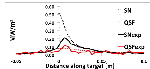
Fig. 2: Head load flux on the outer target: comparison between IR thermography data (solid lines) and TECXY simulation (dashed lines).
