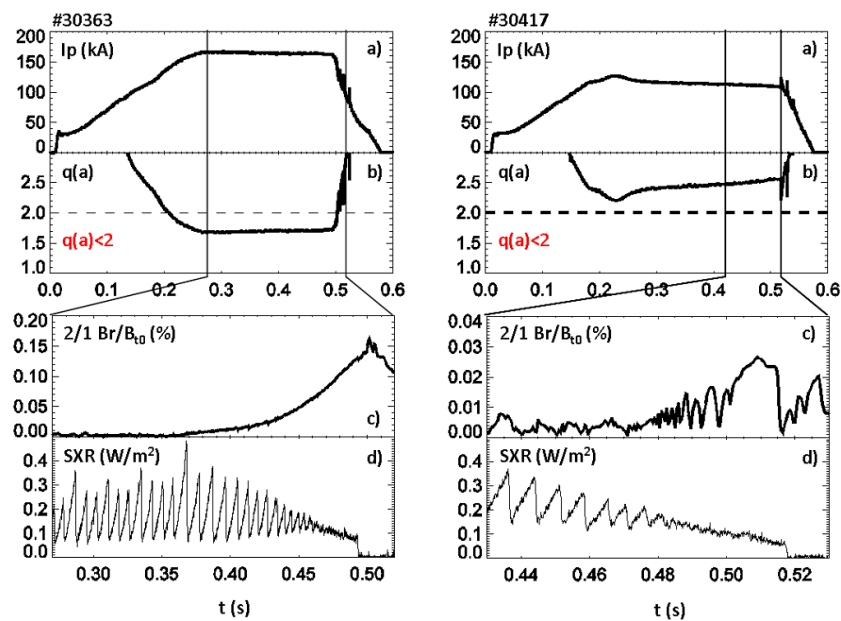
Fig.2 RWM (on the left) and TM (on the right) mitigating effect on sawteeth in RFX-mod. Time history of a) the plasma current, b) the edge safety factor and c) the m=2 , n=1 amplitude of the radial magnetic field normalized to the equilibrium field.
