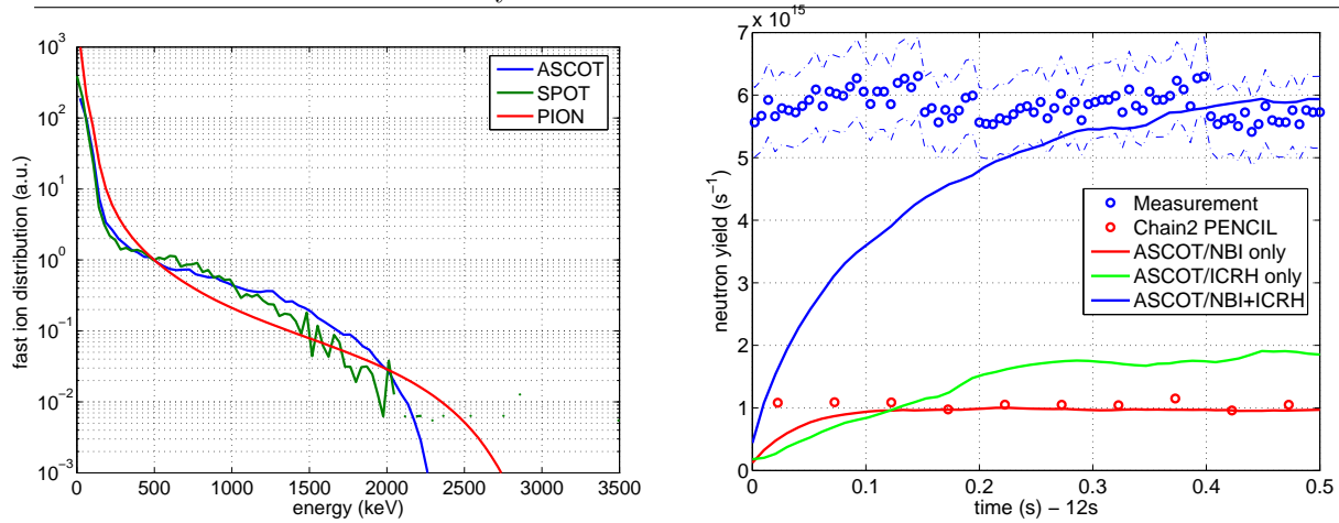
Figure 4: (a) Comparison of normalized fast ion energy distribution between ASCOT/RFOF, SPOT/RFOF and PION. (b) Measured neutron yield in 86459 and ASCOT simulations with NBI, ICRH and NBI+ICRH.
