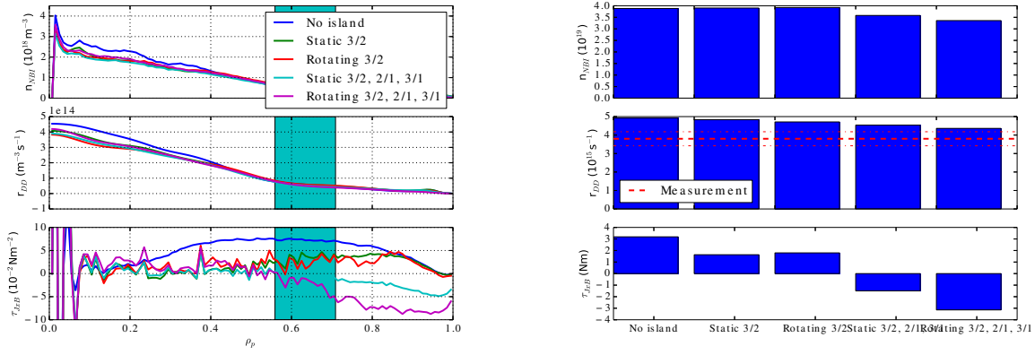
Figure 3: Scan with one or multiple static and rotating islands. (a) profiles of beam ion density, DD neutron rate and beam JxB torque in simulations with static and rotating islands. (b) Volume-integrated values of the profiles. The measured neutron rate is indicated by the dashed red line in the middle panel.
