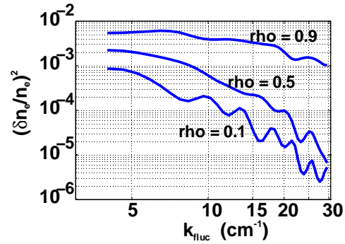
Fig. 2 : Wavenumber density fluctuation spectra calculated at the cut-off positions of Fig. 1 with an integrated radial window of 3.14 cm ( k_{\min}=2\text{cm}^{-1} ).
