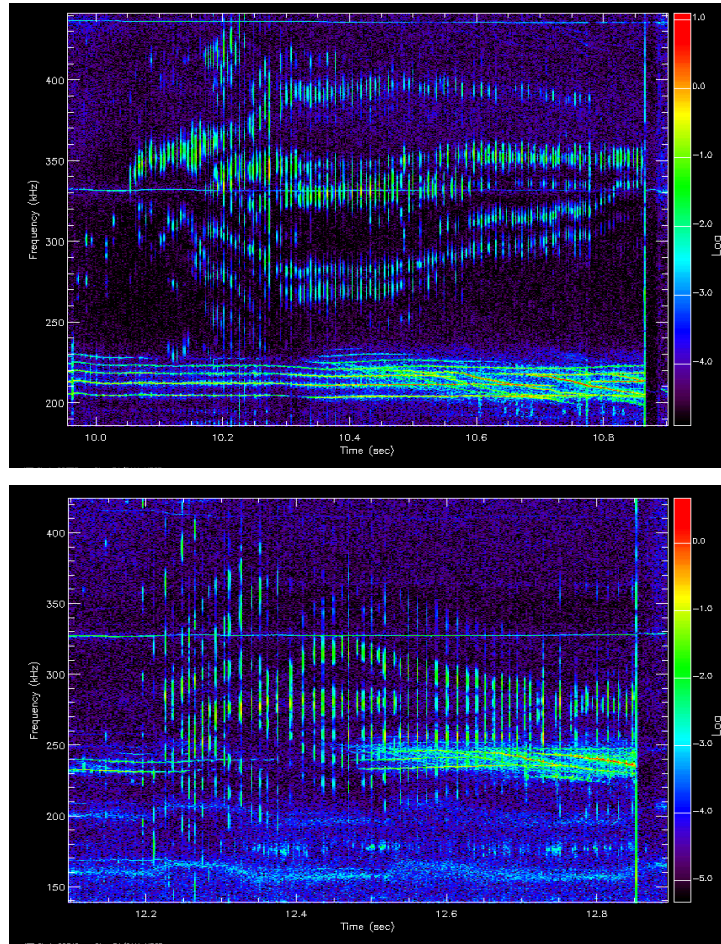
Figure 1: Spectrogram of MHD activity obtained with Mirnov Coils using an acquisition frequency of 1 MHz.
