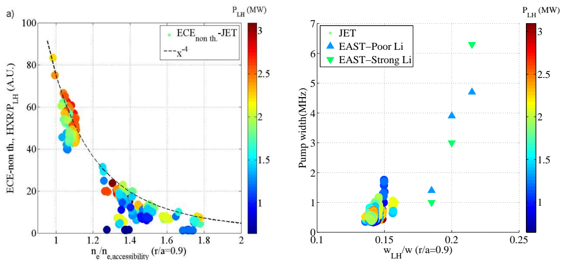
Figure 2. a) \text{ECE}_{\text{non th.}} (JET) as a function of n_e/n_{e,\text{access.}} , b) Pump width at -30\text{dB} (JET), -20\text{dB} (EAST) as a function of \omega_{\text{LH}}/\omega . B_t=1.96\text{--}2.43\text{ T} , N_{//}=1.8 (JET), B_t=2.24\text{ T} , N_{//}=2.1 (EAST).
