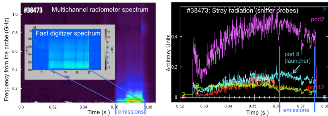
Fig.2: Left: Multichannel radiometer and fast digitizer spectra during pulses. Right: Sniffer probes signals show a relatively higher stray radiation measured at the launcher port 8 in coincidence with intense spectral emissions.
