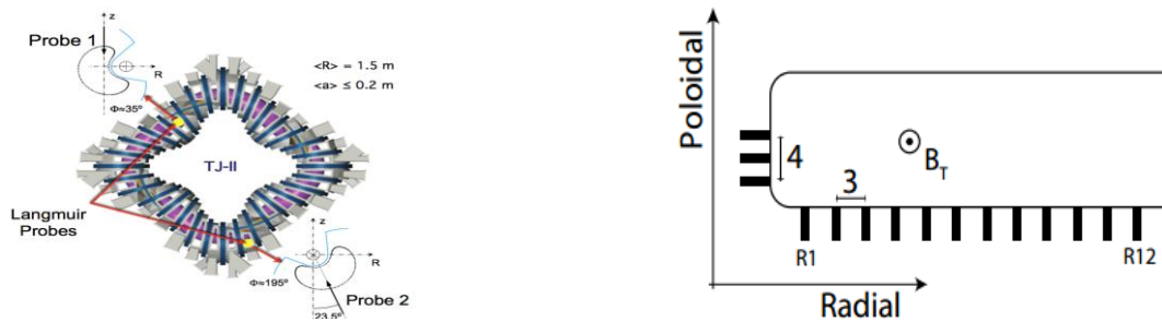
Fig. 1: a) Placement of the two rake probes in the TJ-II stellarator. b) Representation of one of the rake probes (probe 1)
