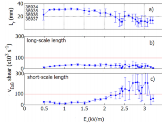
Fig. 3: Radial correlation, global and local E_r shearing rates versus the long scale radial electric field.
