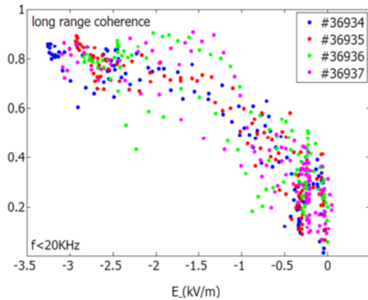
Fig. 2: Amplitude Long Range Correlations versus the long scale radial electric field (global E_r ) for low frequencies ( f < 20 \text{ KHz} ).
