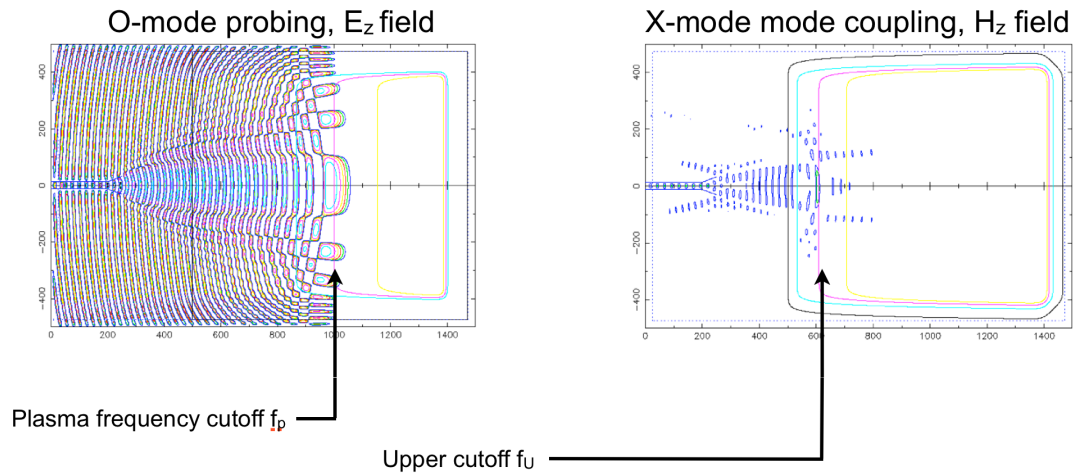
Figure 2: O -mode is excited on the TM_z plane, being reflected at the plasma frequency f_p . Signal is coupled to X -mode propagating until reaching the upper branch frequency cutoff f_u .
