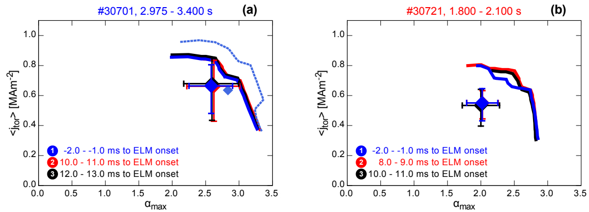
Figure 3: j - \alpha diagrams for phases in which the high frequency fluctuations are present: (a) #30701, for comparison the light-blue dashed boundary is calculated from a CLISTE equilibrium [10], and (b) #30721. For the analysed time intervals, stability boundaries and operational points are similar.
