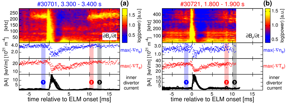
Figure 1: Pedestal evolution for high ((a), #30701) and low collisionality ((b), #30721): ELM-synchronised spectrogram of \partial B_r/\partial t and ELM-synchronised time traces of \max(-\nabla n_e) (blue), \max(-\nabla T_e) (red) and inner divertor current (black). The vertical bars and numbers indicate the phases in which the linear MHD stability analyses were performed. In both discharges, after \max(-\nabla T_e) is recovered (10 ms (#30701) respectively 8 ms (#30721) after the ELM onset) fluctuations set in. Figures modified from [6].
