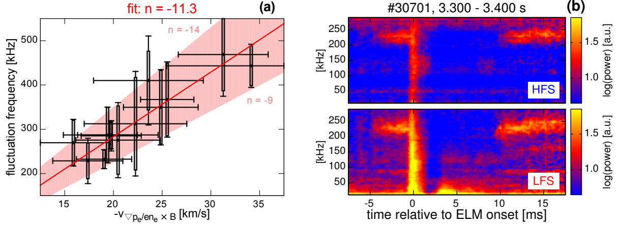
Figure 2: Neoclassically estimated background velocity and comparison of LFS and HFS fluctuations: (a) fluctuation frequency over -v_{\nabla p_e / e n_e} (\propto v_{E \times B}) . From the linear dependence between the detected fluctuation frequency and the background flow velocity a toroidal mode number n of approximately -11 can be determined (red line). (b) Spectrogram of the HFS (top) and the LFS ballooning coil signals. The high frequency fluctuations are also detected on the HFS. Figure modified from [6].
