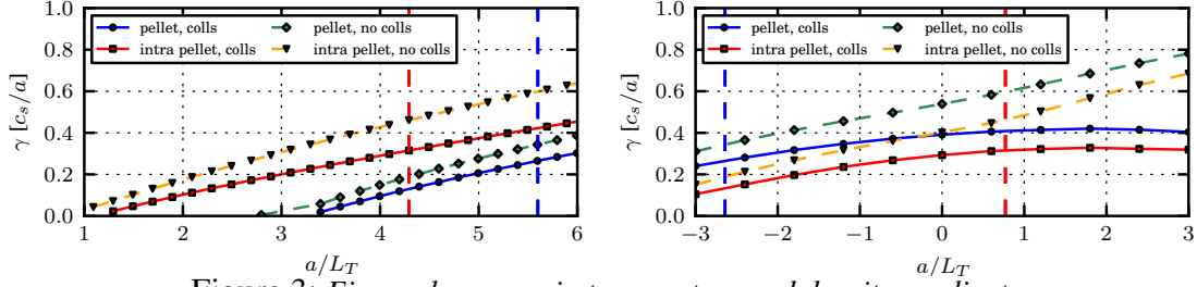
Figure 3: Eigenvalue scans in temperature and density gradients
