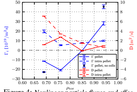
Figure 4: Nonlinear particle fluxes and effective diffusion coefficients.
