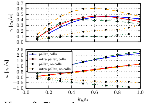
Figure 2: Eigenvalue spectra at \rho_{\text{tor}} = 0.69 , subdominant modes dotted.
