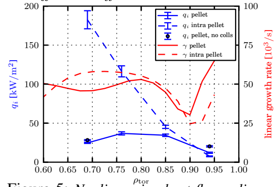
Figure 5: Nonlinear ion heat fluxes, linear growth rates at k_y \rho_s = 0.3 also shown.
