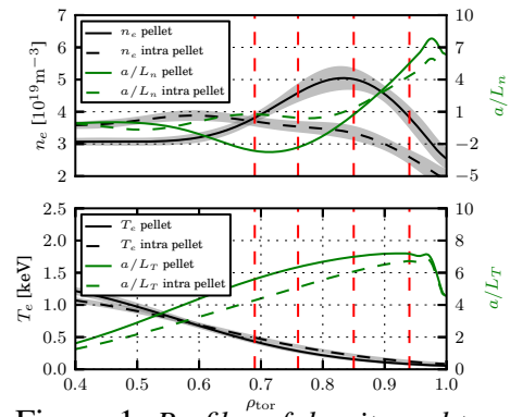
Figure 1: Profiles of density and temperature. Dashed lines indicate radial positions of the NL analysis.
