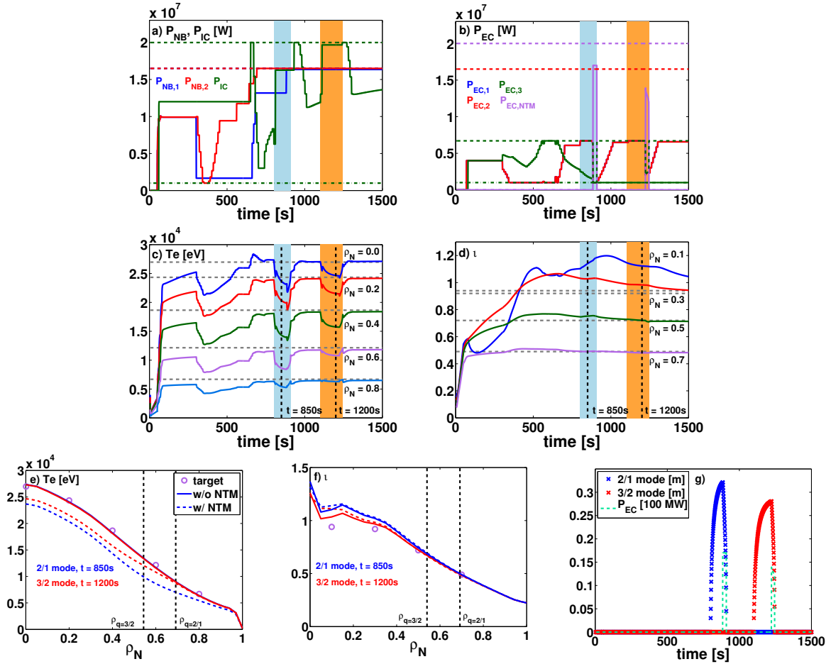
Figure 2: Time trace of a) NB, IC, b) EC powers with the maximum (dashed) and minimum (dashed dot) power limits and c) T_e and d) \tau profiles with target (dashed). The coloured boxes indicate the appearance of NTMs (light blue - 2/1 mode, orange - 3/2 mode). e), f) T_e and \tau profiles are shown in comparison with those without NTM. The island size of each mode and applied EC power are presented in g).
