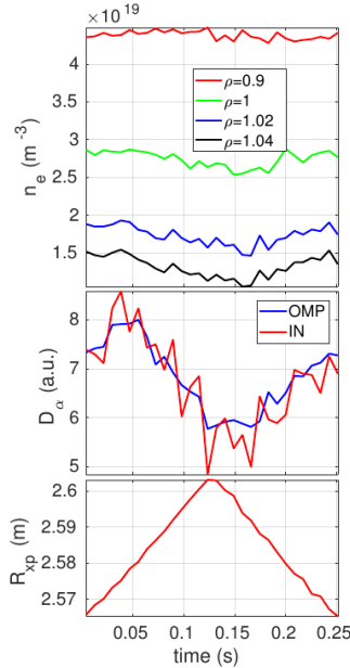
Figure 4 Coherently averaged signals for one full sweep (4 Hz) show midplane electron density from reflectometer (top), D_\alpha line of sight measurement at the midplane and at the inner divertor apron (middle) and the X-point major radius location (bottom). See Fig. 1 for 'IN' location.
