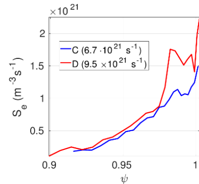
Figure 8 Flux surface averaged neutral ionisation source density and totals in the legend.
