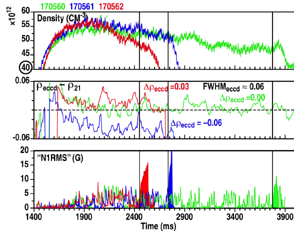
Fig. 6. Preemptive CW EC at q\sim 2 . j_{\text{eccd}}/j_{\text{boot}}\sim 0.8 and dP_{\text{ecrh}}/dV\sim 7*P_{\text{nbi}}/V with 4 gyrotrons of 2.2 MW. a) density evolution, b) alignment target varied, c) n=1 Mirnov. Verticals 2/1 onset. In this set, q=2 aiming delays mode onset the longest; ECRH-only 170563 (not shown) also delays mode similarly to 170560.
