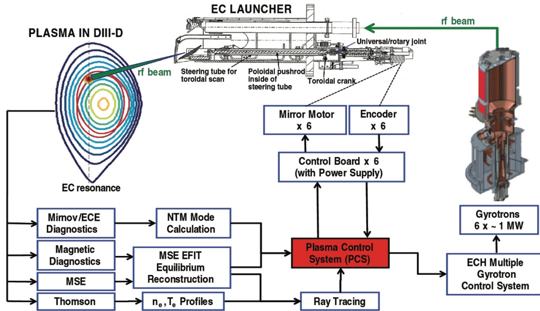
Fig. 4. Schematic of DIII-D real-time ECCD tearing mode control system as now fully implemented. Each of up to 6 gyrotrons on a separate mirror can be independently directed to separate q -surfaces. Up to 8 in 2019.
