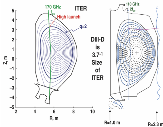
Fig. 5. Cross-sections of ITER and of a DIII-D ITER Baseline Scenario discharge showing the launch of rays (170 GHz 1*f_{\text{ec}} and 110 GHz 2*f_{\text{ec}} respectively) to drive co-ECCD at q=2 .
