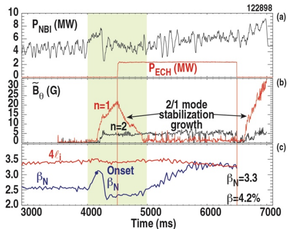
Fig. 3. (a) NBI and EC powers; (b) the n=1 (red) and n=2 (black) components of the Mirnov at the outer midplane of the vacuum vessel; (c) internal inductance multiplied by 4 (red) and normalized beta (blue).
