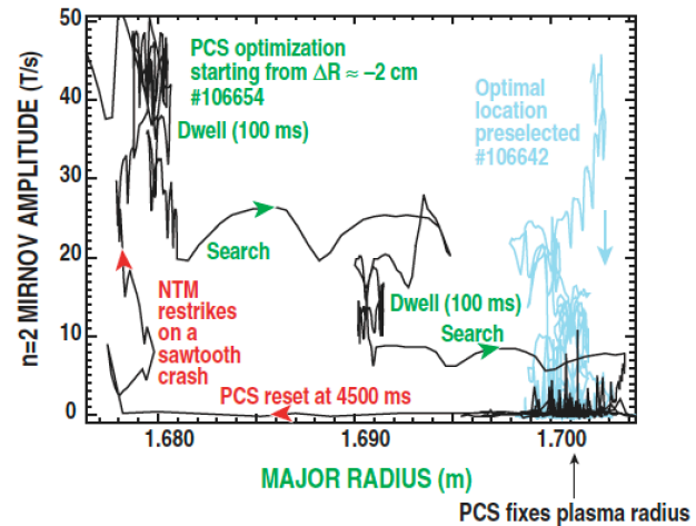
Fig. 2. Real-time PCS control of major radius to put the q-surface for m/n=3/2 on the location of the ECCD. PCS dwells to see response and if mode not stabilized searches by stepping radius, dwells etc until stability, then freezes until reset to starting radius at preprogrammed time.
