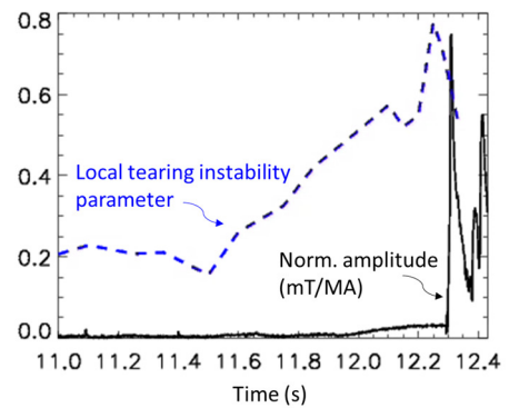
Figure 2: Time evolution of the computed local tearing instability parameter at q=2 (in blue) and the normalized mode amplitude (in black) of the baseline plasma reported in figure 1.
