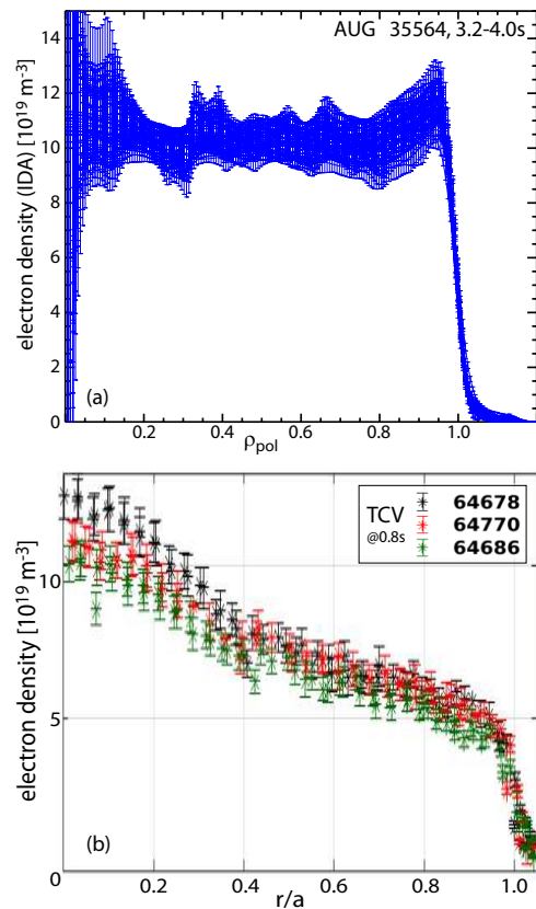
Fig. 2: Comparison of typical density profiles from ITER BLS in TCV and AUG.
