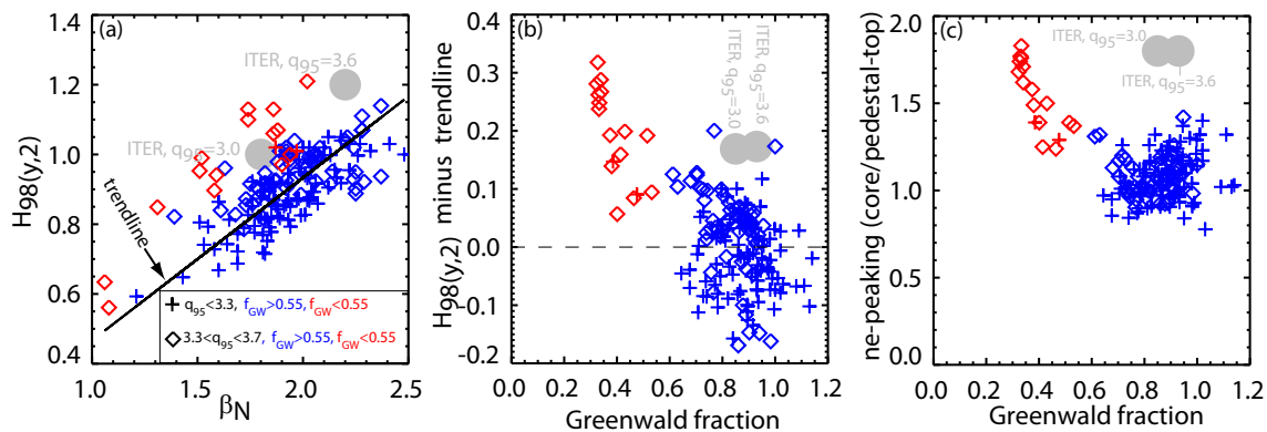
Fig. 1: Trends in global parameters for the ITER BLS discharges in AUG. More details in the text.
