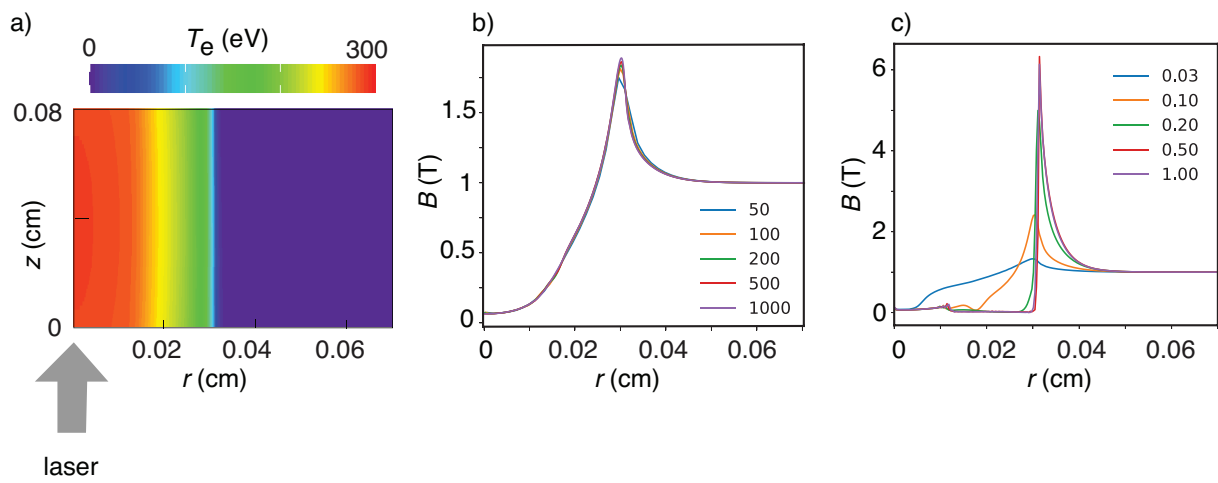
Figure 1: Test problem to validate Nernst term treatment: laser heated low density gas, with parameters as in Sec. II of Ref. [12] and initial uniform magnetic of 1 T (along z ). a) Electron temperature map at the end of the laser pulse ( t = 0.5 ns); b) radial profiles of magnetic field at z = 0.04 cm, for different radial meshing and the same Nernst flux limiter f_N = 0.07 ; the curve labels indicate the number of radial mesh points N_r ; c) same as b), but for different values of f_N (labeling the curves), and for N_r = 200
