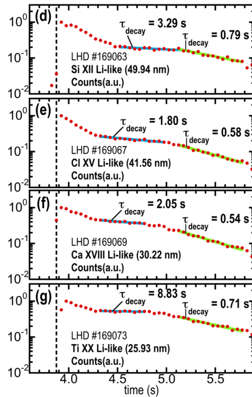
Fig.4. Temporal evolutions of the (a) CX Li III, (b) CX B V, and (c) CX Al XIII emissions measured with the CXS technique. And temporal evolutions of (d) Si Li-like, (e) Cl Li-like, (f) Ca Li-like, (g) Ti Li-like emissions measured with the SOXMOS spectrometer. These are obtained in the high-density LHD plasmas. The vertical dashed line indicates the TESPEL injection time. All the Li-like emissions are normalized by the maximum during the time period shown.
