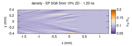
Figure 1: Electron density from HERA .
