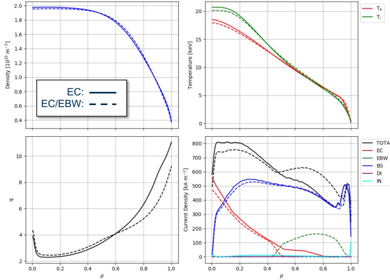
Figure 2: Profiles of the two preferred FTOPs using either pure ECDD (solid) or combined ECDD/EBW heating.
