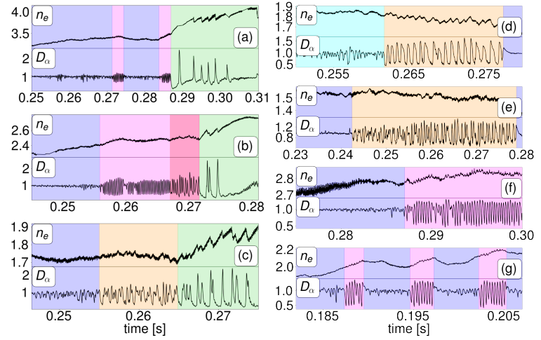
Figure 1: n_e [ 10^{19}\text{m}^{-3} ] and D_\alpha traces showcasing the categories used in the P_{LH} studies. Left: H-modes at different densities (decreasing from (a) to (c)), with (a) showing a typical H-mode, (b) a long pre-H i-phase and (c) a dithery H-mode. Boundary behaviours are shown on the right, with dithery periods in (d) and (e) and i-phases in (f) and (g).
