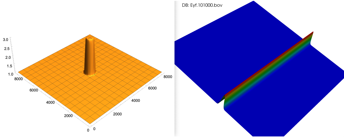
Figure 1: (a) the dielectric cylinder n(x, z) , (b) The E_y of the initial electromagnetic pulse .
