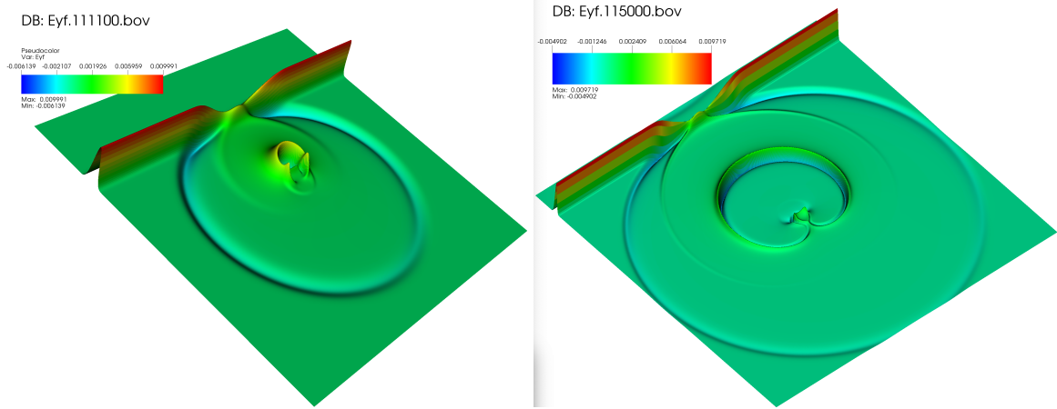
Figure 3: (a) Later stages of scattering of E_y , (b) The E_y(x,z,t) at the end of the QLA simulation.
