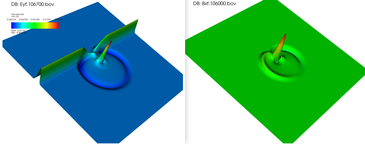
Figure 2: (a) Early stage of scattering of E_y , (b) The generation of B_x field
