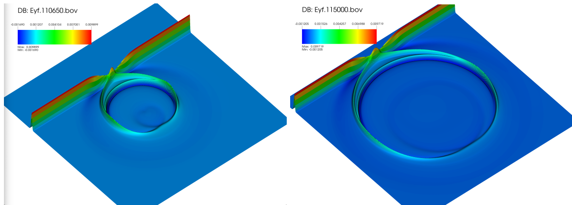
Figure 4: (a) Early stage of scattering of E_y , (b) The E_y(x,z,t) at the end of the QLA simulation.
