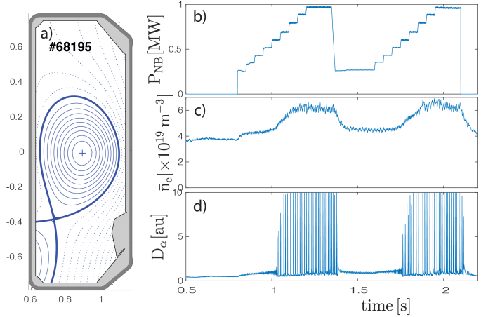
Figure 1: Experimental scenario with a) plasma shape, b) neutral beam heating power, c) line averaged density and d) D_\alpha emission.
