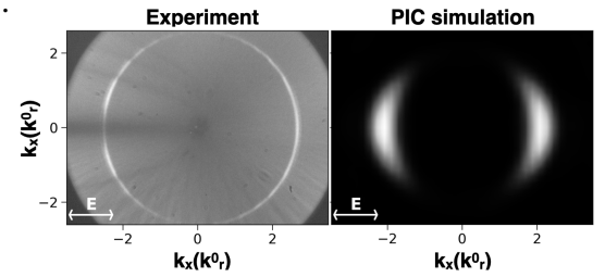
Figure 1: Second-harmonic spatial spectrum from experiment versus simulation. k_r^0 = k_0 \sin \theta where \theta is the cone angle.
